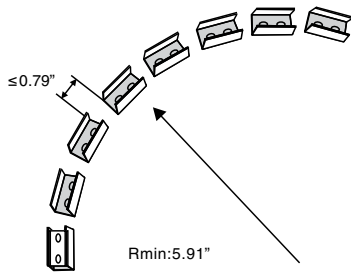
Plastic Profile Joint Horizontally
