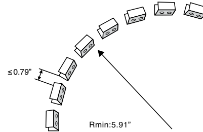
Plastic Profile Joint Vertically
