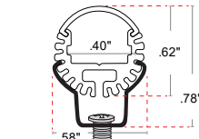
Profile with Stainless Steel Mounting Clip
