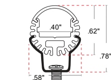
Profile with Stainless Steel Mounting Clip
