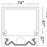
Profile with Hidden Stainless Steel Mounting Clip
