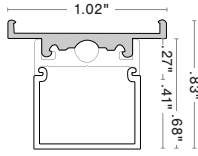
Profile with Plastic T-Bar Mounting Clip
